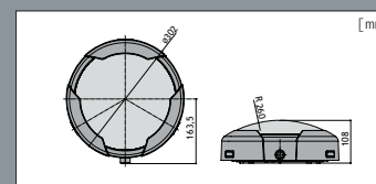
DROP 1 LED
