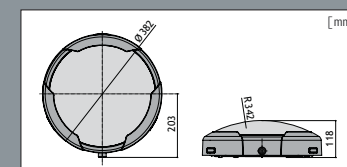
DROP 2 LED
